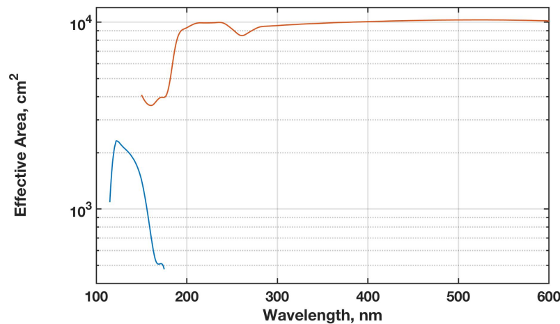
Figure 7: Effective area of the FCU
